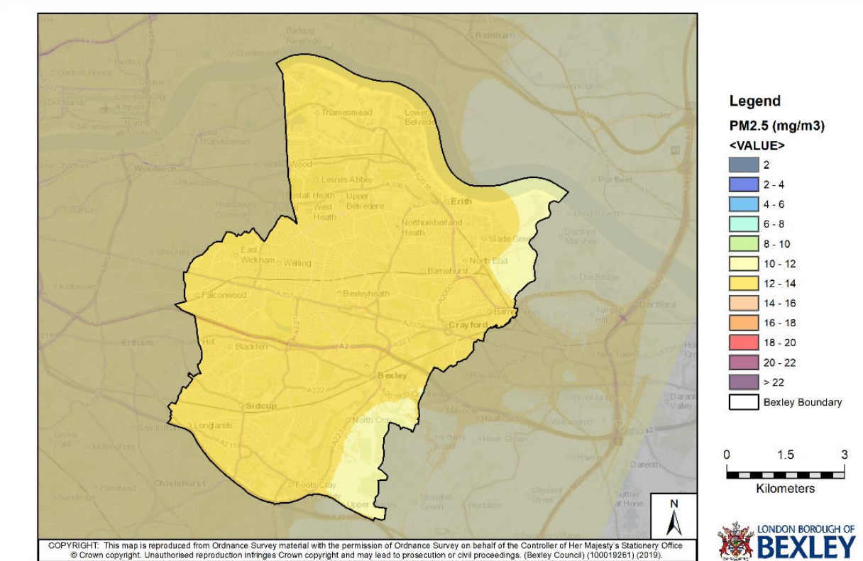
Fig. 3.18: Annual Mean PM2.5 concentrations (London Atmospheric Inventory 2016)
